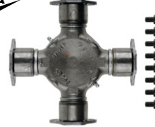
U-Joint, Greaseable, 1810 Series. DS5281X
